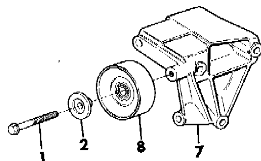
2.5L ENGINE
